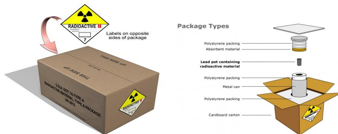
Figure 6.1: Radioactive package and 3-levels of containment
